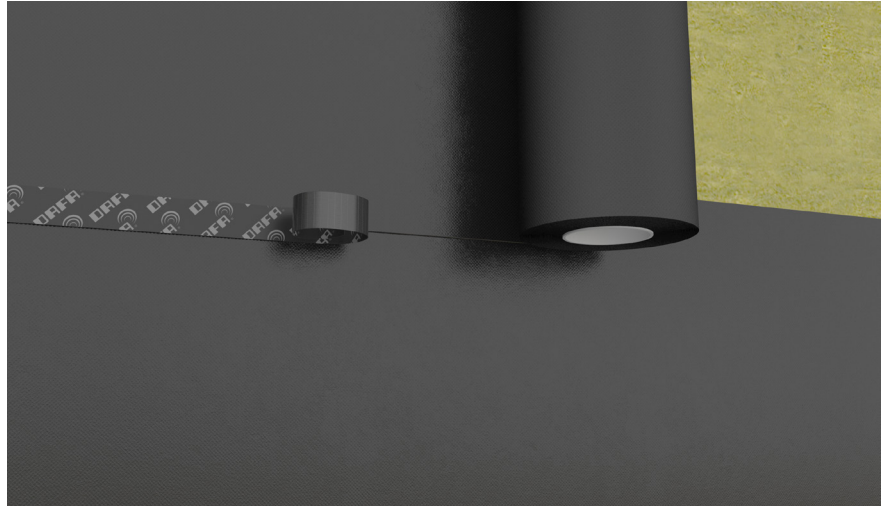
DAFA UV facade is installed as a wind barrier with a minimum overlap of 150 mm and free joints are taped using DAFA UV tape.
