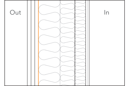
DAFA UV facade is used as a wind barrier with a ventilated cavity behind the rainshield.
