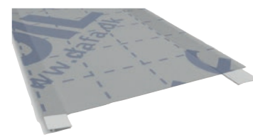
5 DAFA lining foil with groove - interior sealing of door and window apertures.
