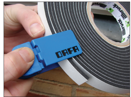
11. The roll should be secured tightly using the self-adhesive locking tape (or DAFA's sealing tape clip) and stored lying horizontally at around 19°C. This will ensure that the sealing tape does not expand whilst being stored.
