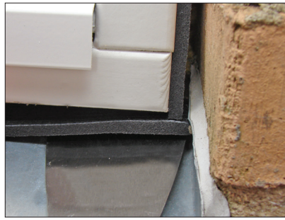
8. The horizontal piece of sealing tape is put in place and pressed together with the vertical piece (see illustration 8).
