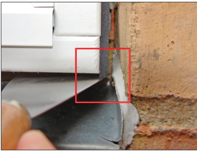
7. For corner joints, the vertical piece should be placed 1-2 mm beyond the horizontal piece.
