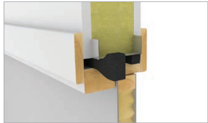
Sound absorption with illmod 600 sealing tape in door structures, between the steel profile and the frame.
