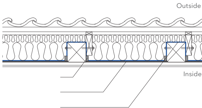
DAFA HiFoil is leveled out against DAFA IsoBatt and across the existing rafters. The membrane is fixed to the rafter with DAFA counter-batten.
