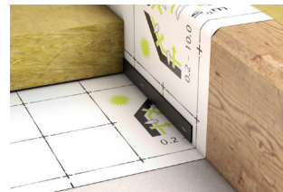
DAFA HiFoil is leveled out against DAFA IsoBatt and across the existing rafters. The membrane is fixed to the rafter with DAFA counter-batten.
