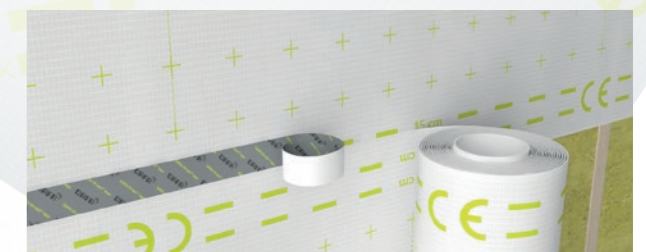
DAFA ExFoil consists of polyethylene (PE) material with reinforcing mesh in the middle and a moisture-absorbing polypropylene (PP) fleece layer. The material can withstand direct sunlight for up to three months, and must not be exposed to direct contact with wood preservative with added solvents.
