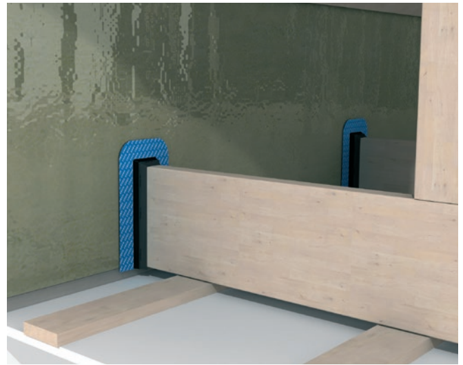
DAFA rafter shoe collar
