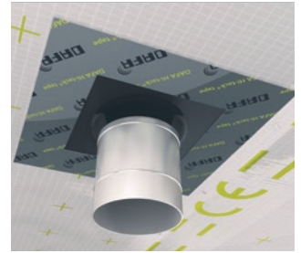
DAFA Hi-tack® pipe collars are used for DAFA ExFoil and DAFA HiFoil vapor barriers.
