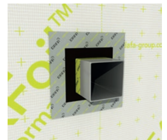
DAFA Hi-tack® pipe collars are used for DAFA ExFoil and DAFA HiFoil vapor barriers.
